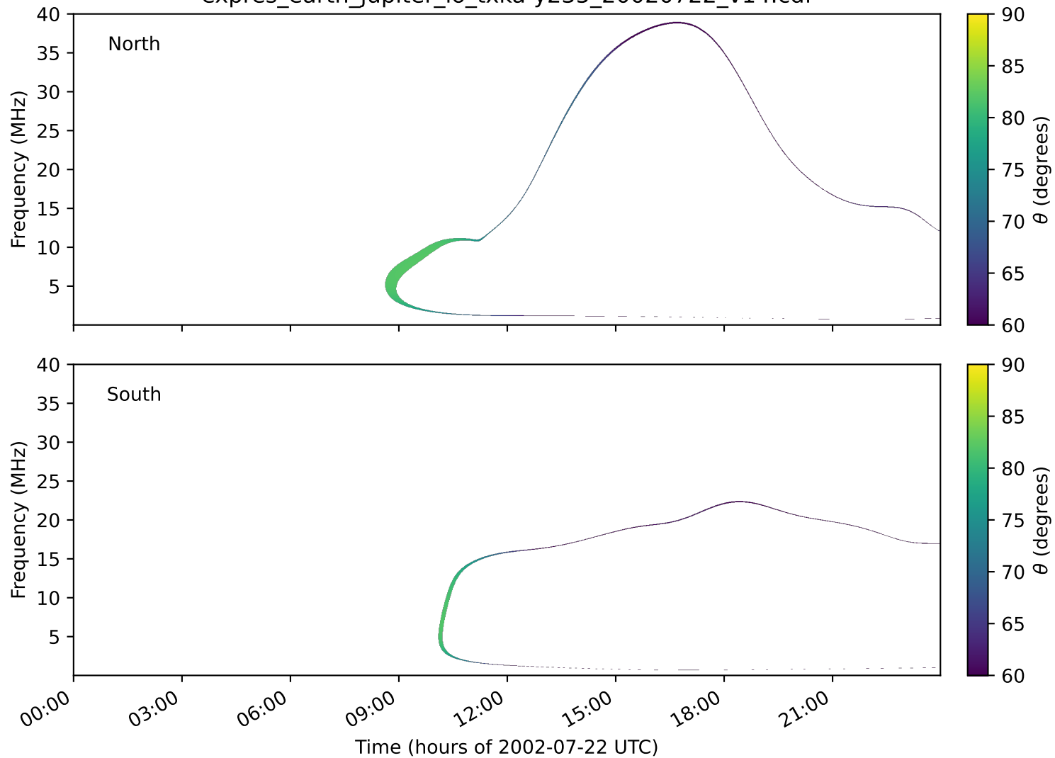
expres_earth_jupiter_io_txka-y235_20020722_v14.cdf
