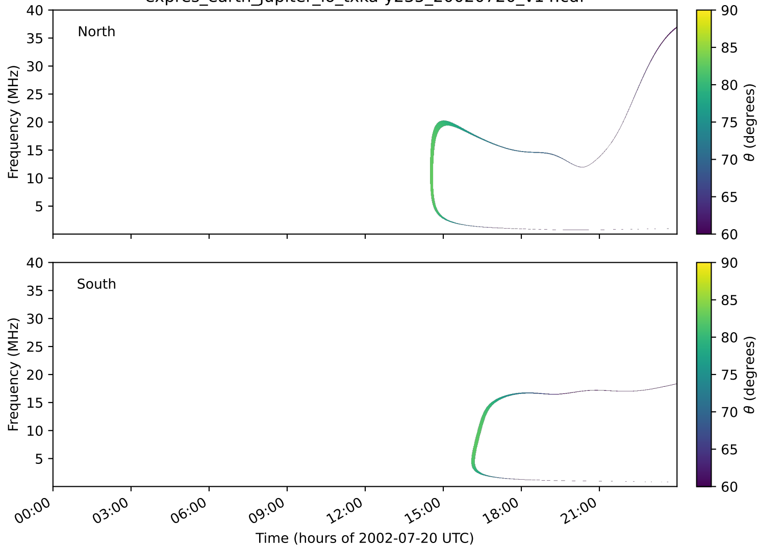
expres_earth_jupiter_io_txka-y235_20020720_v14.cdf
