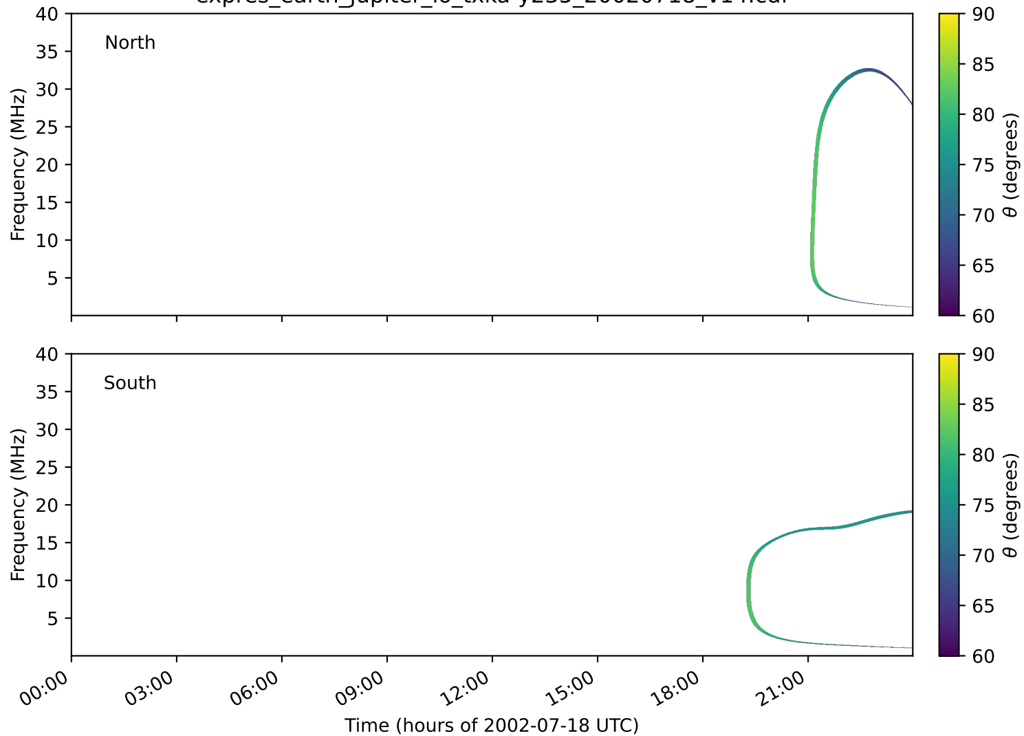
expres_earth_jupiter_io_txka-y235_20020718_v14.cdf
