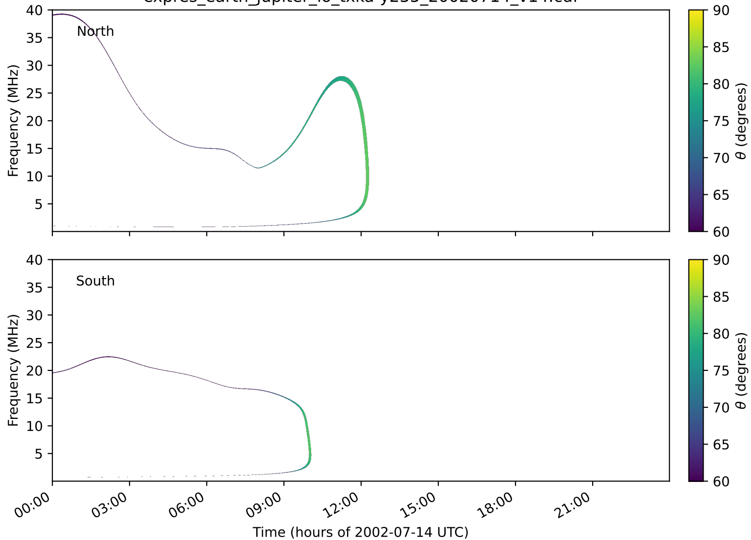
expres_earth_jupiter_io_txka-y235_20020714_v14.cdf
