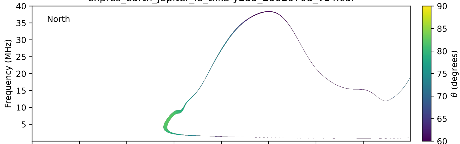
expres_earth_jupiter_io_txka-y235_20020708_v14.cdf
