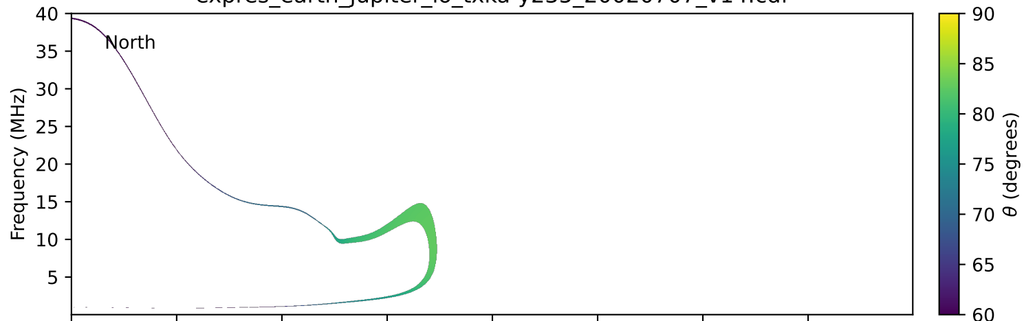
expres_earth_jupiter_io_txka-y235_20020707_v14.cdf
