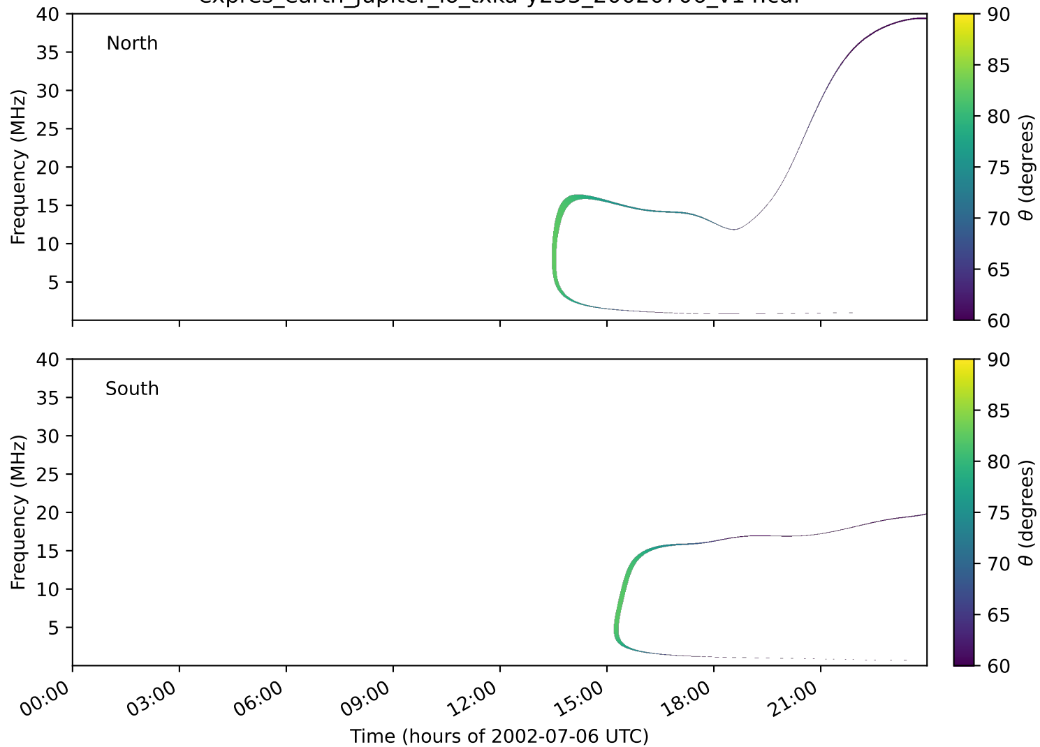
expres_earth_jupiter_io_txka-y235_20020706_v14.cdf
