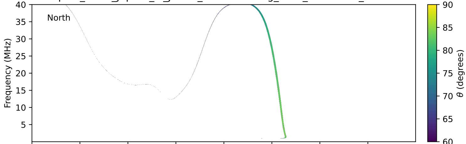
expres_earth_jupiter_io_jrm33_lossc-wid1deg_3kev_20020728_v11.cdf
