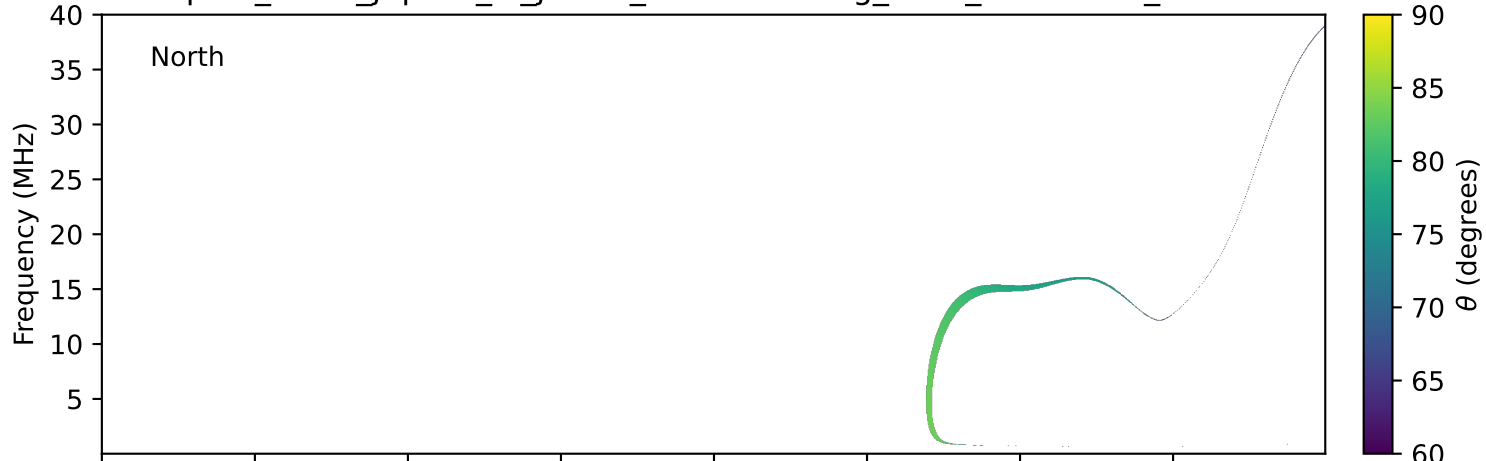
expres_earth_jupiter_io_jrm33_lossc-wid1deg_3kev_20020727_v11.cdf
