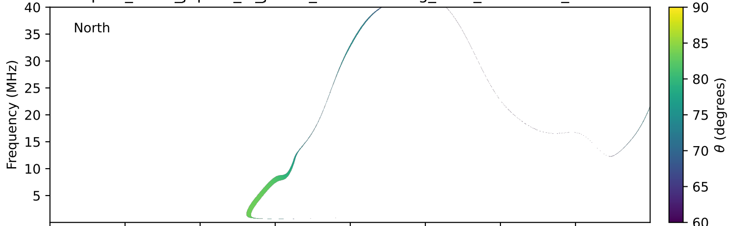
expres_earth_jupiter_io_jrm33_lossc-wid1deg_3kev_20020708_v11.cdf
