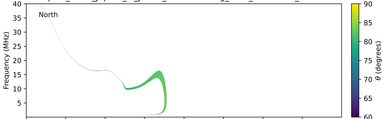
expres_earth_jupiter_io_jrm33_lossc-wid1deg_3kev_20020707_v11.cdf
