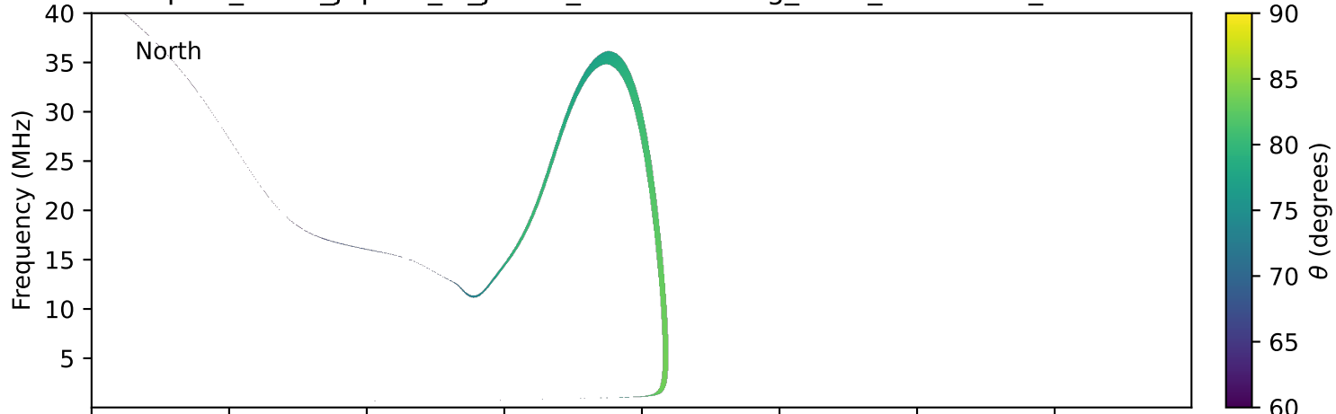
expres_earth_jupiter_io_jrm09_lossc-wid1deg_3kev_20020714_v11.cdf
