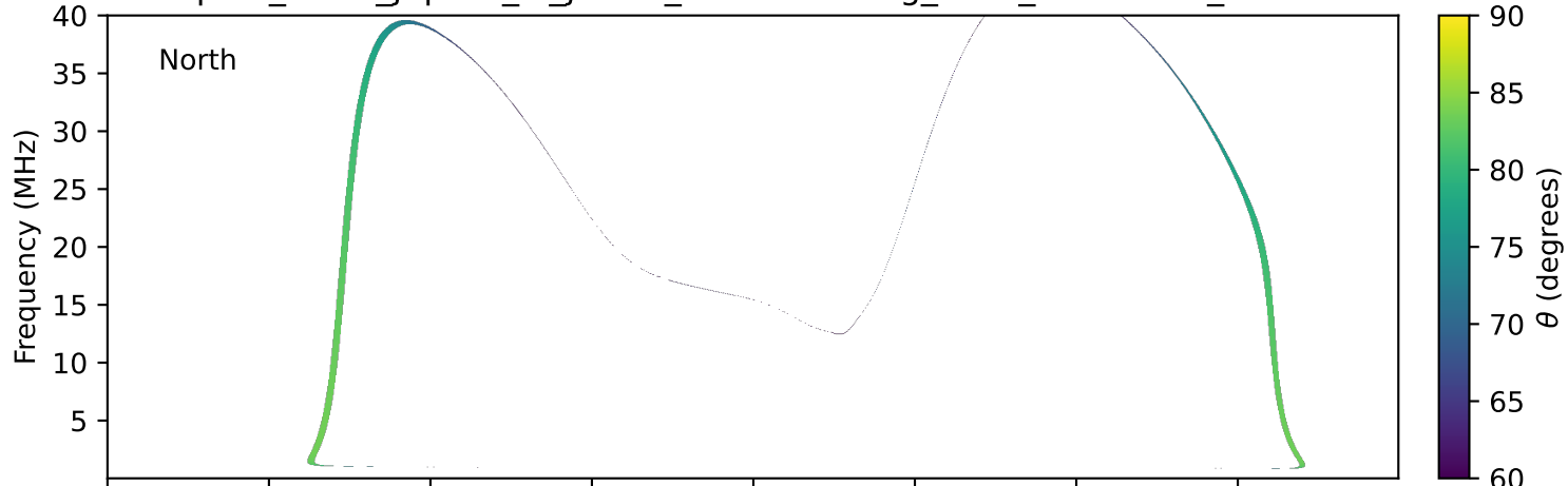
expres_earth_jupiter_io_jrm09_lossc-wid1deg_3kev_20020710_v11.cdf
