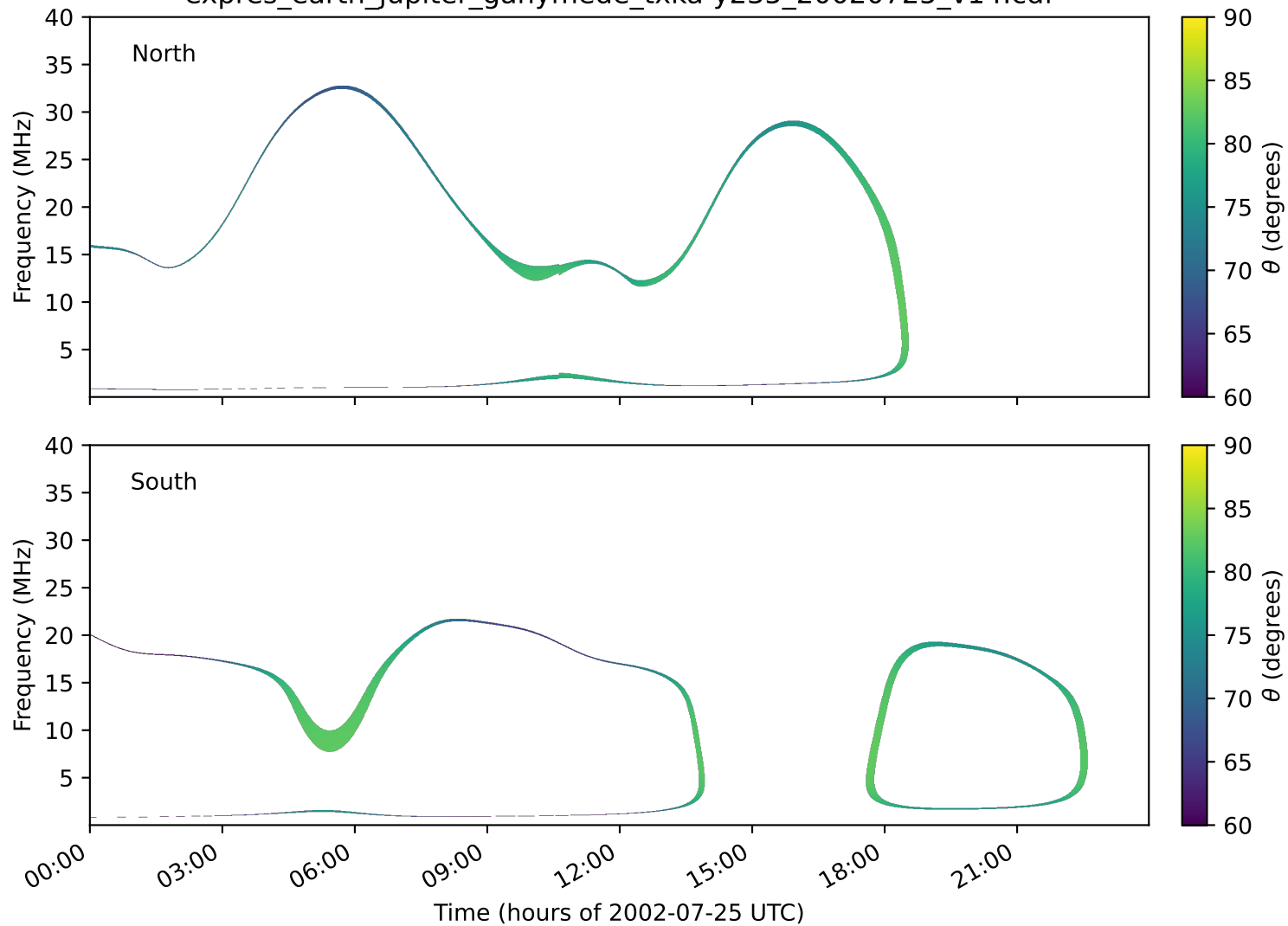
expres_earth_jupiter_ganymede_txka-y235_20020725_v14.cdf
