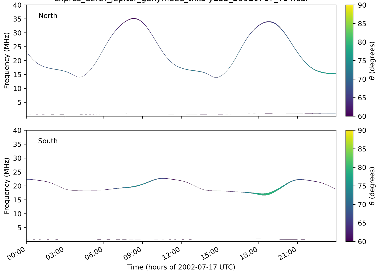
expres_earth_jupiter_ganymede_txka-y235_20020717_v14.cdf
