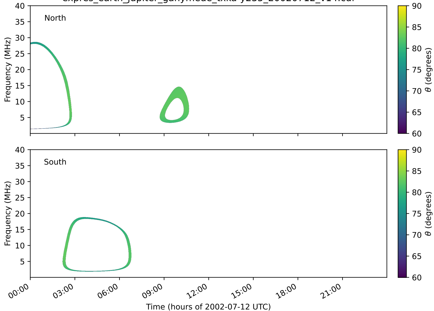
expres_earth_jupiter_ganymede_txka-y235_20020712_v14.cdf
