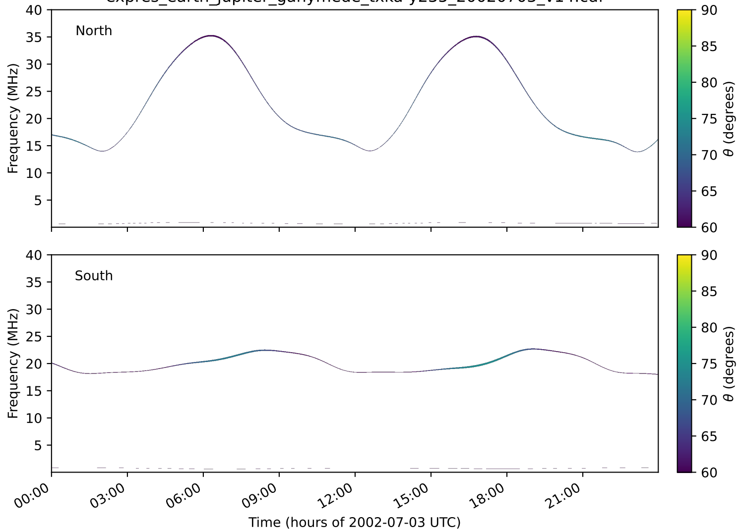
expres_earth_jupiter_ganymede_txka-y235_20020703_v14.cdf
