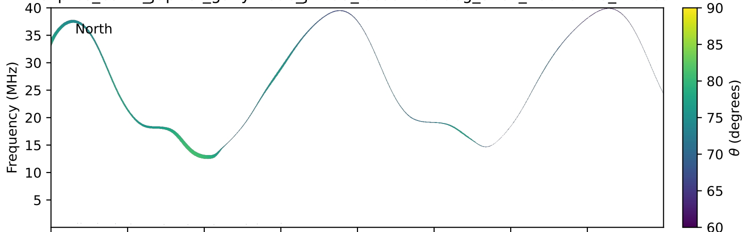
expres_earth_jupiter_ganymede_jrm33_lossc-wid1deg_3kev_20020716_v11.cdf
