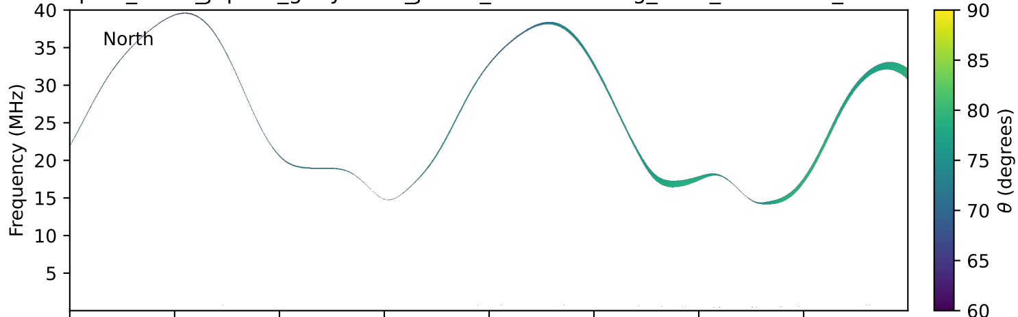
expres_earth_jupiter_ganymede_jrm33_lossc-wid1deg_3kev_20020704_v11.cdf
