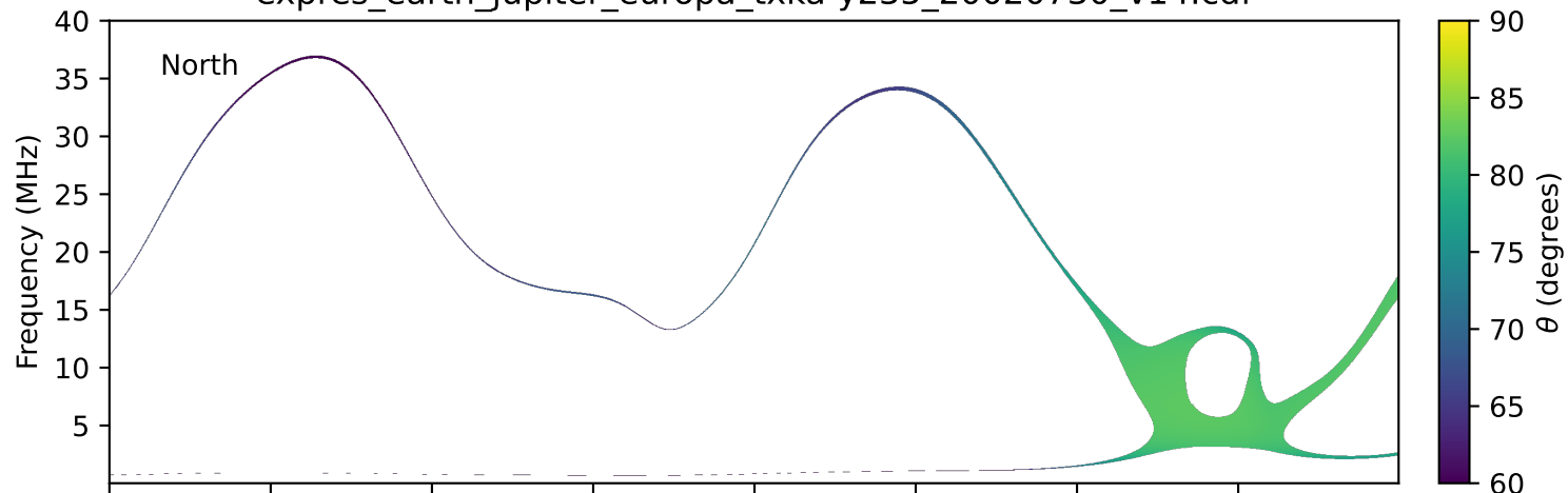
expres_earth_jupiter_europa_txka-y235_20020730_v14.cdf
