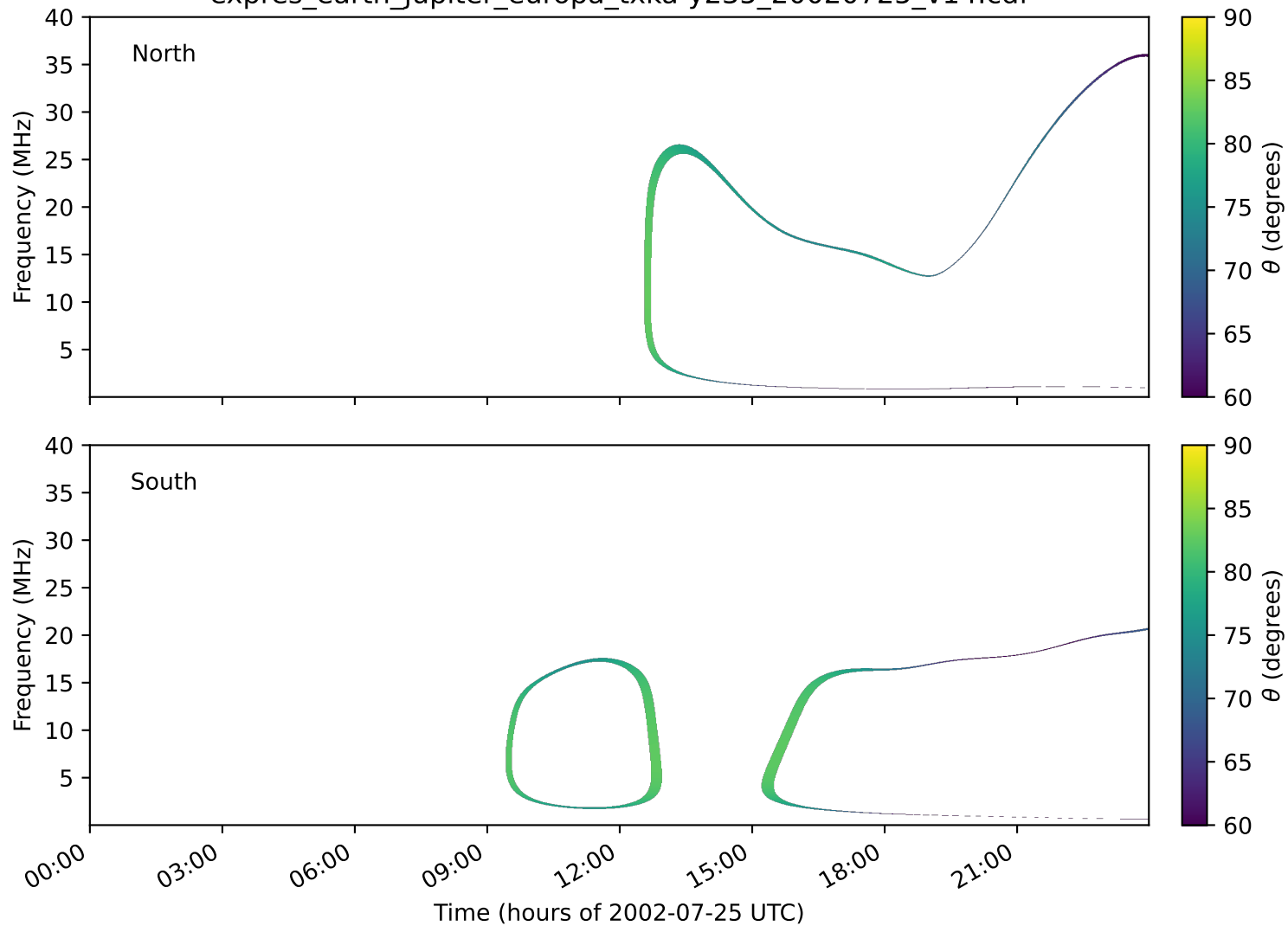
expres_earth_jupiter_europa_txka-y235_20020725_v14.cdf
