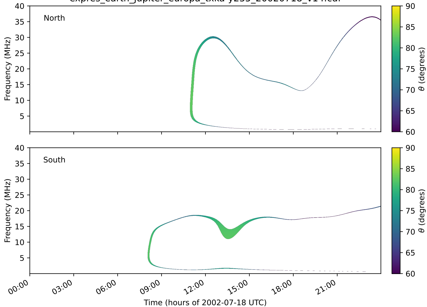
expres_earth_jupiter_europa_txka-y235_20020718_v14.cdf
