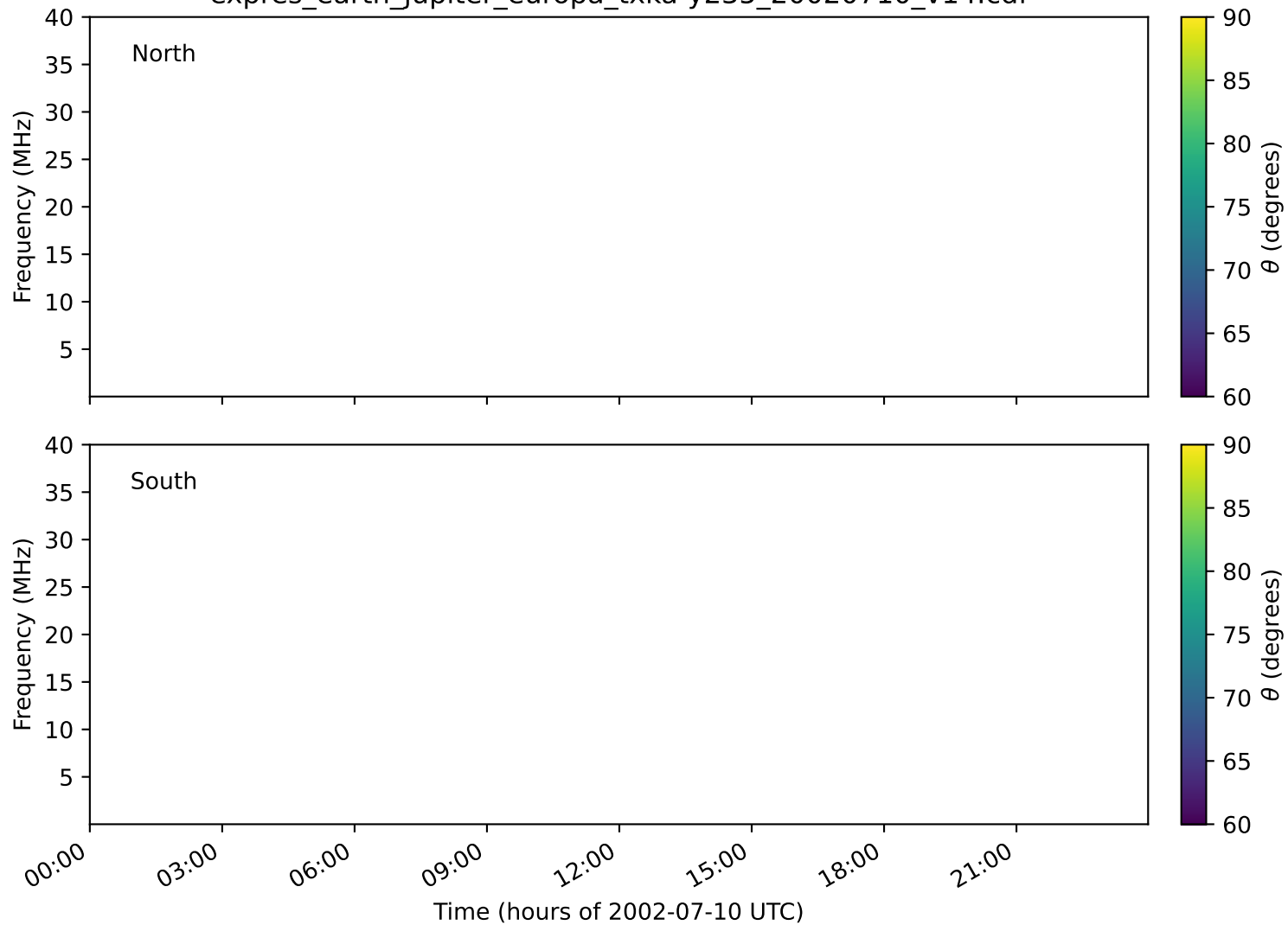
expres_earth_jupiter_europa_txka-y235_20020710_v14.cdf
