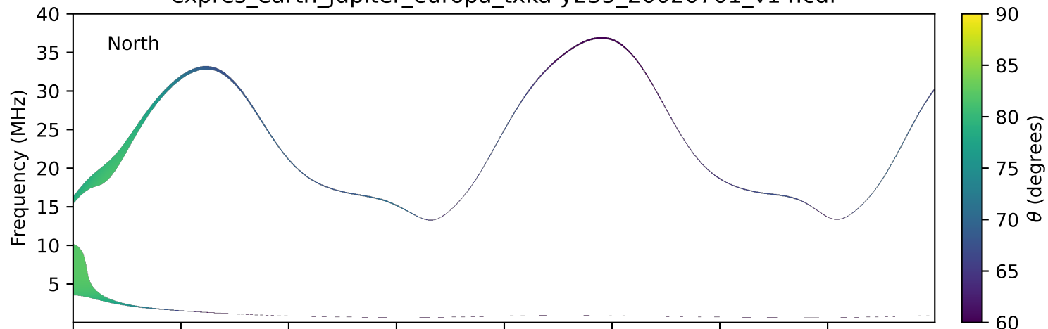
expres_earth_jupiter_europa_txka-y235_20020701_v14.cdf
