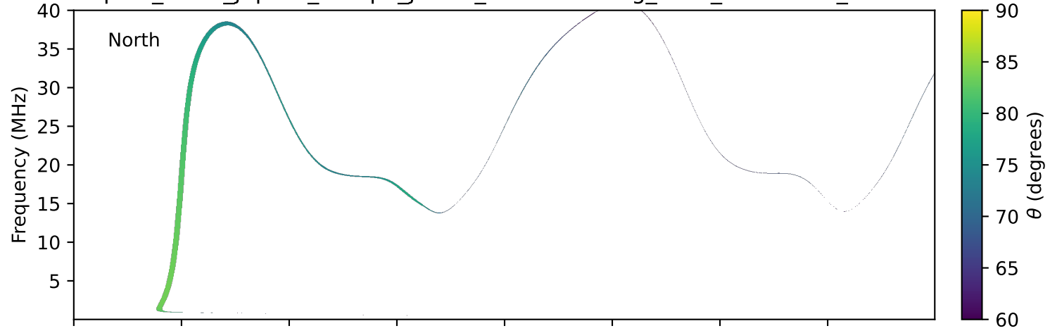
expres_earth_jupiter_europa_jrm33_lossc-wid1deg_3kev_20020708_v11.cdf
