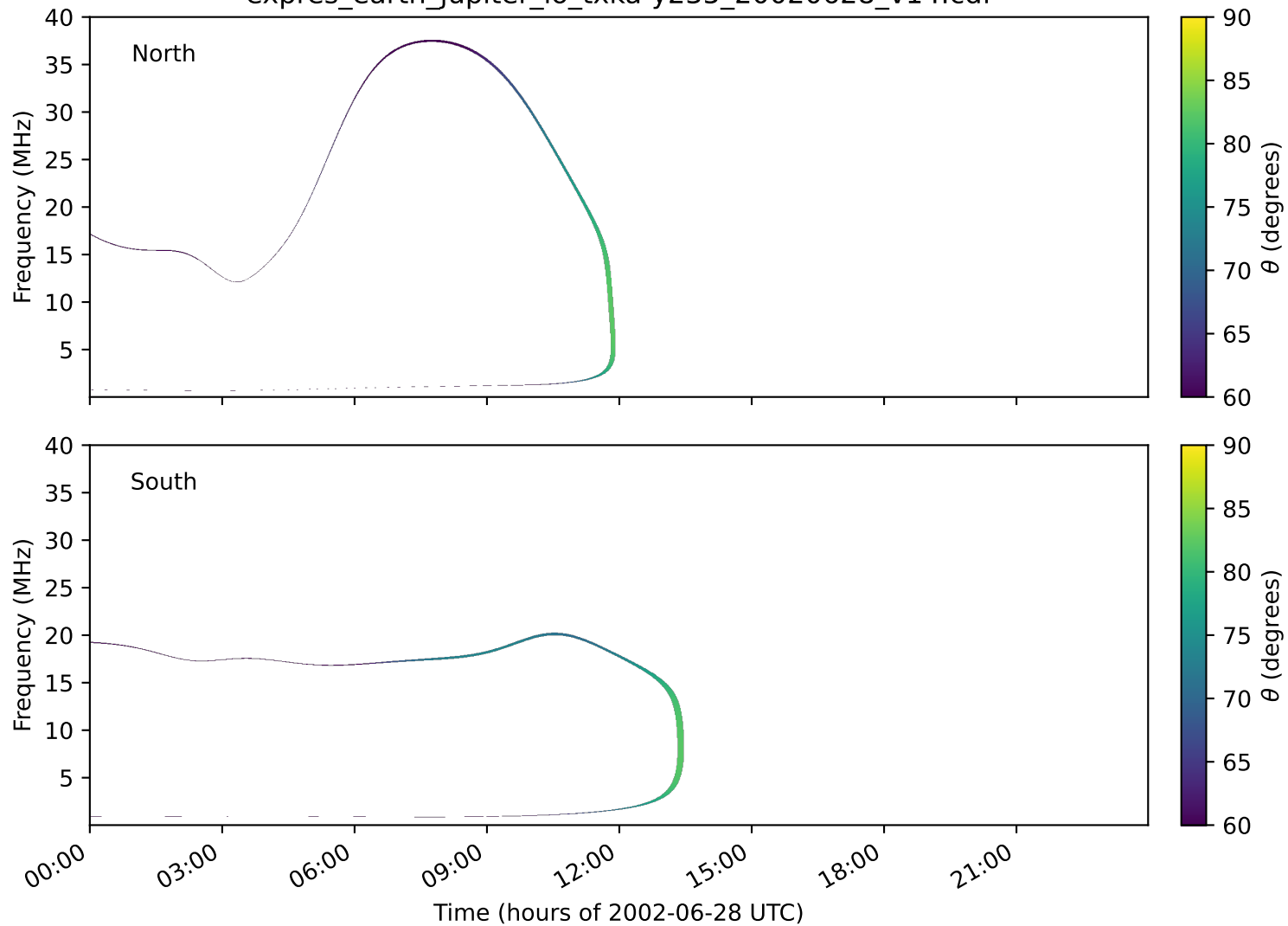
expres_earth_jupiter_io_txka-y235_20020628_v14.cdf
