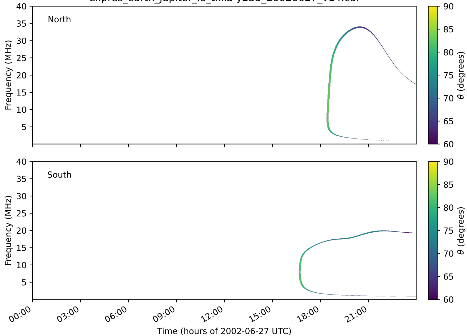
expres_earth_jupiter_io_txka-y235_20020627_v14.cdf
