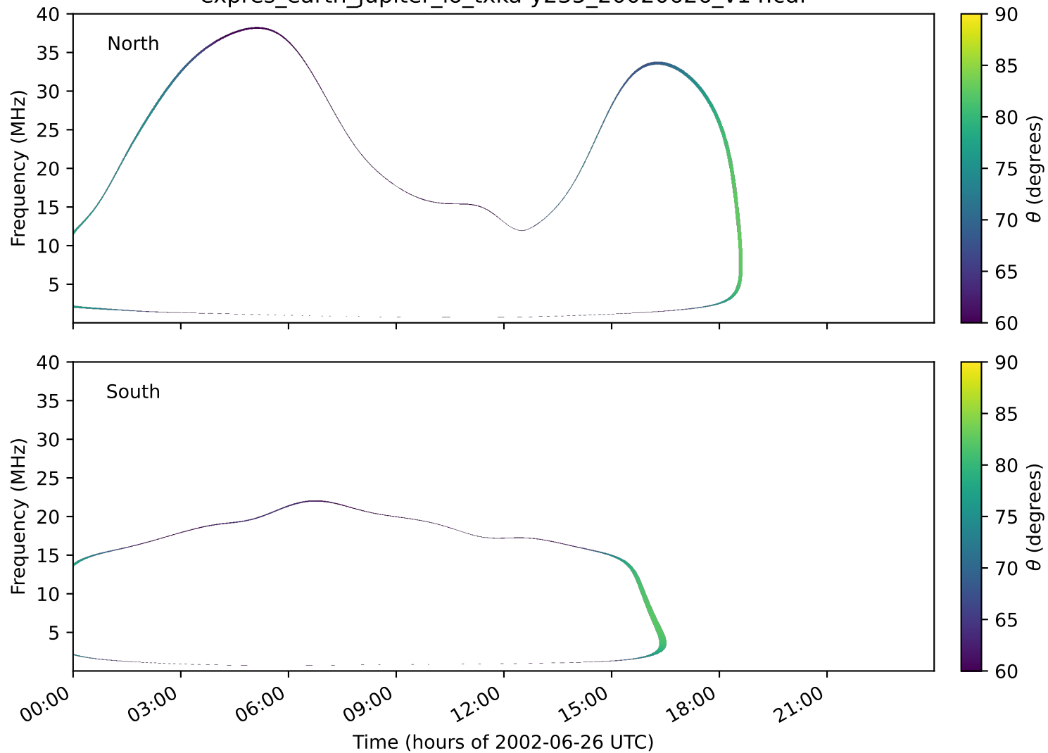
expres_earth_jupiter_io_txka-y235_20020626_v14.cdf
