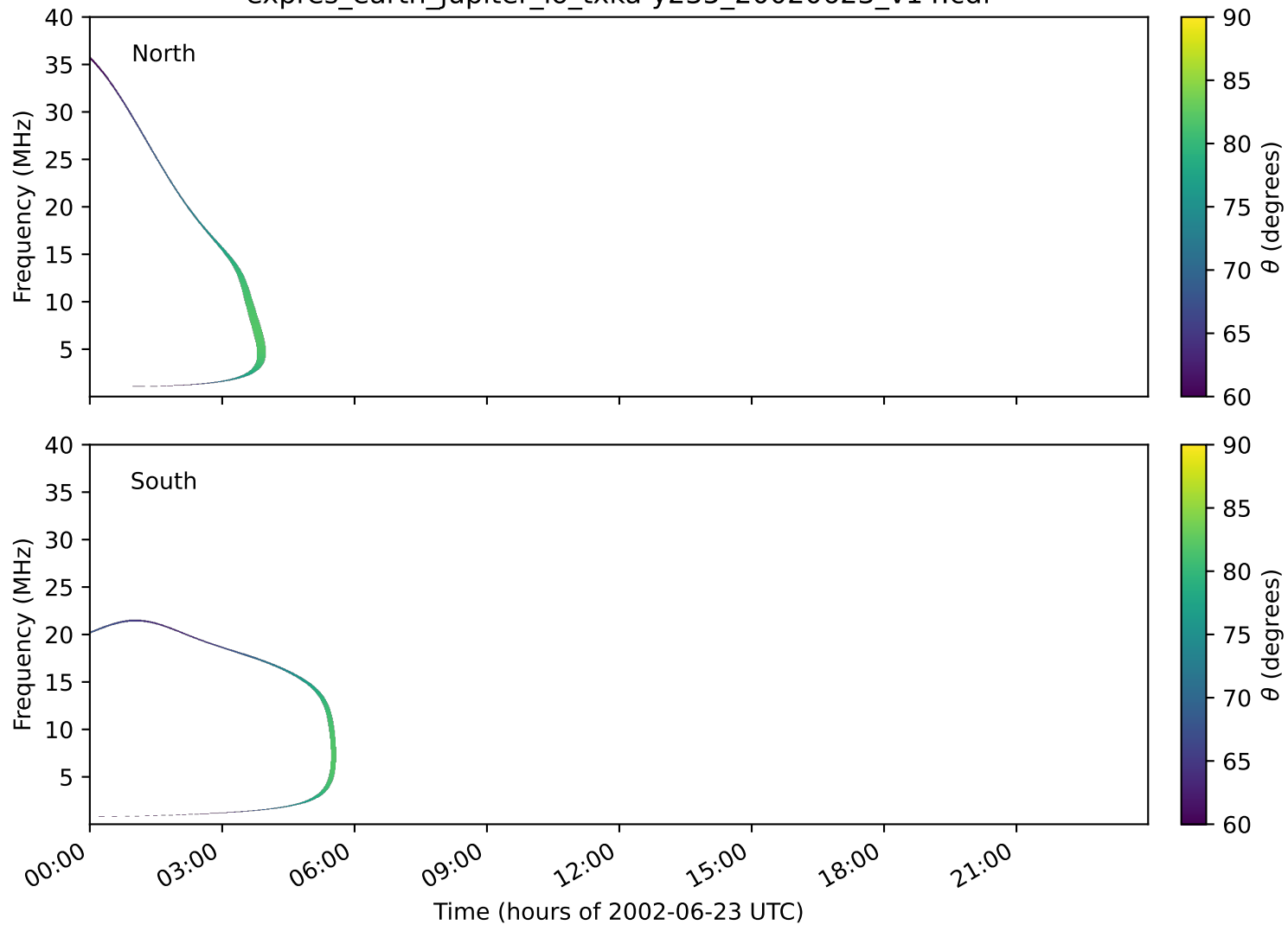
expres_earth_jupiter_io_txka-y235_20020623_v14.cdf
