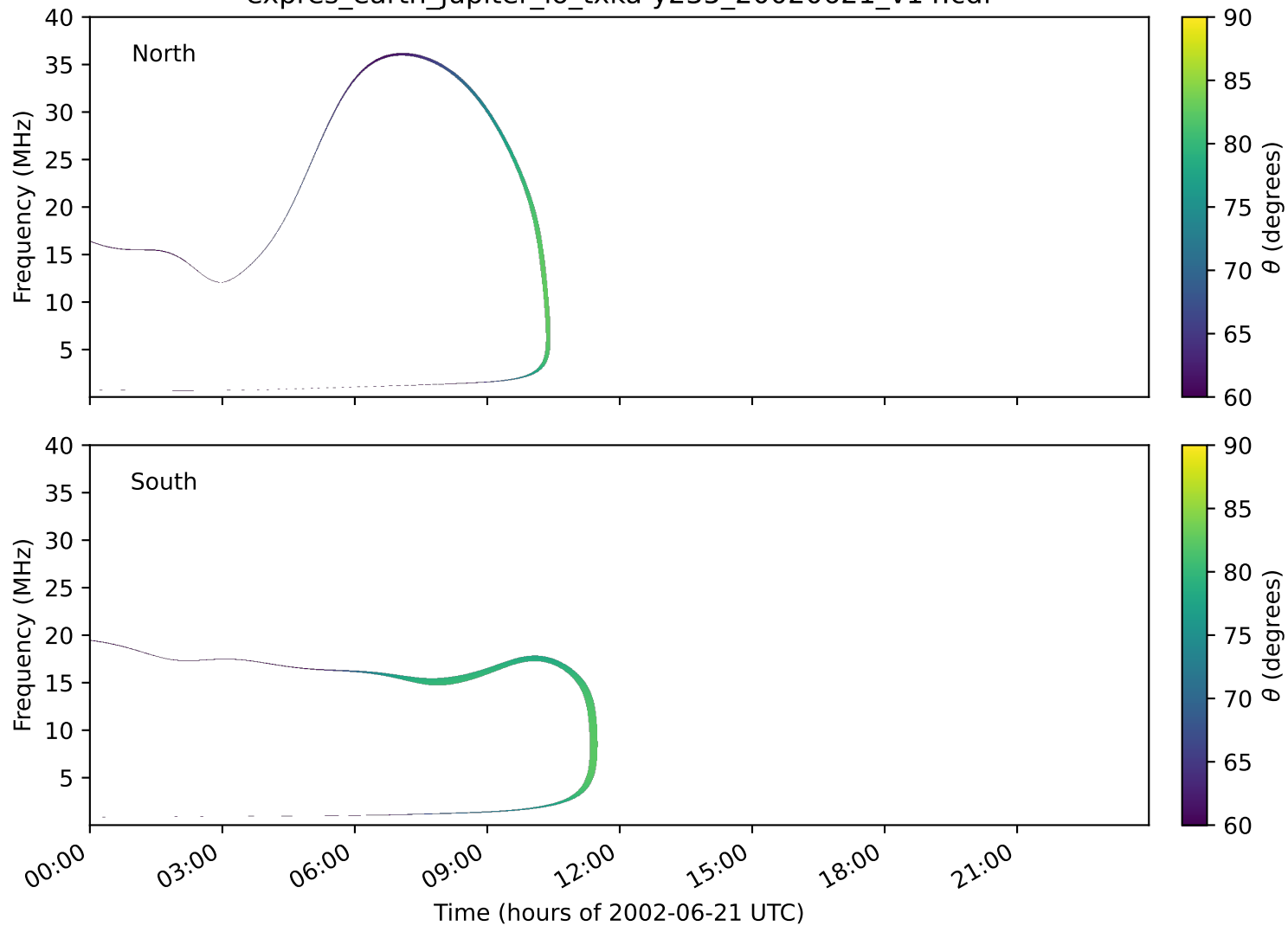
expres_earth_jupiter_io_txka-y235_20020621_v14.cdf
