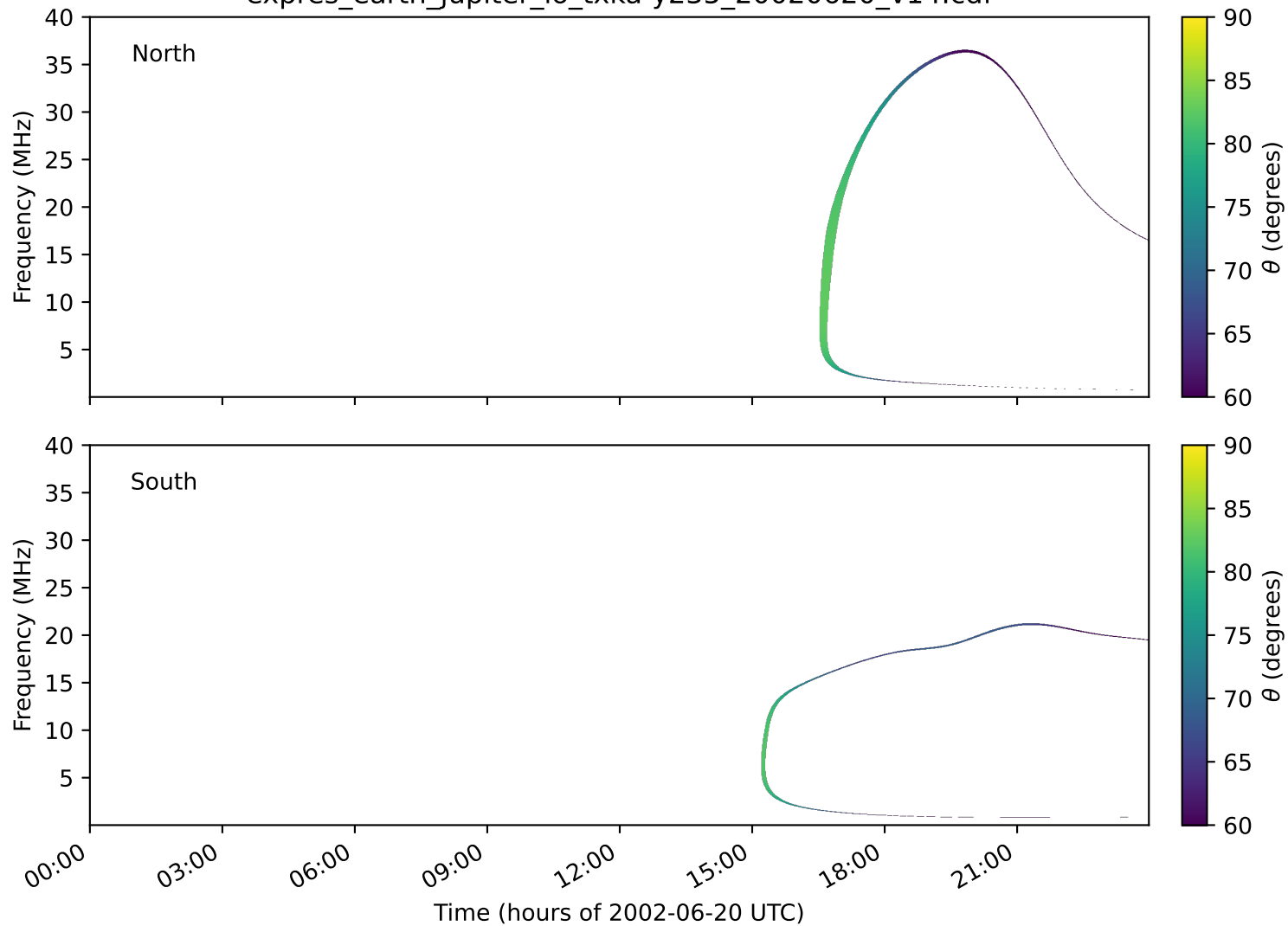
expres_earth_jupiter_io_txka-y235_20020620_v14.cdf
