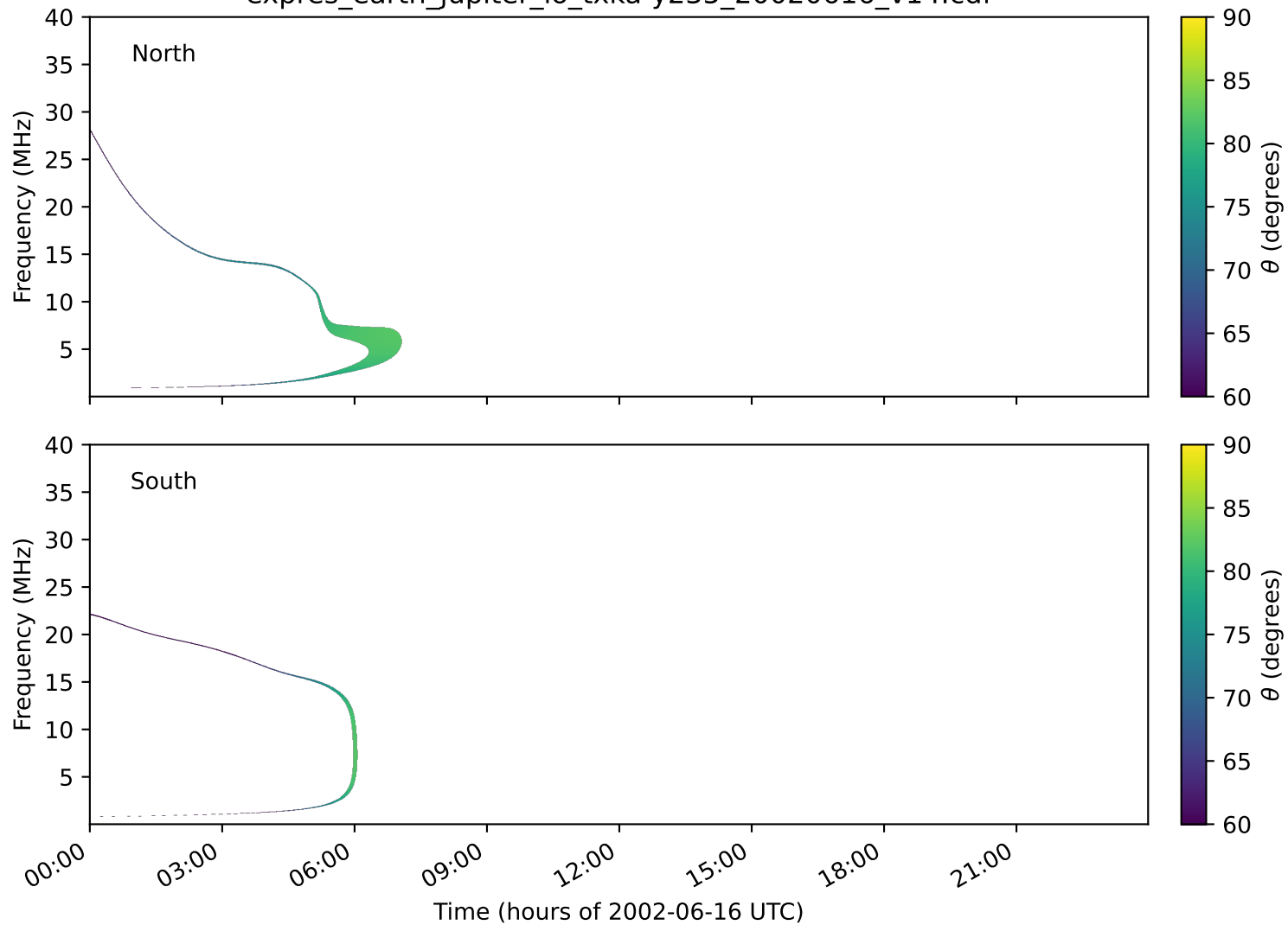
expres_earth_jupiter_io_txka-y235_20020616_v14.cdf
