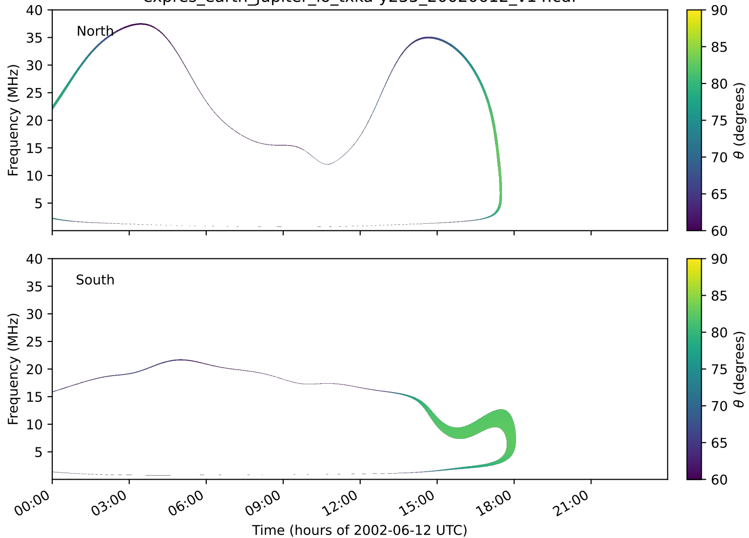
expres_earth_jupiter_io_txka-y235_20020612_v14.cdf
