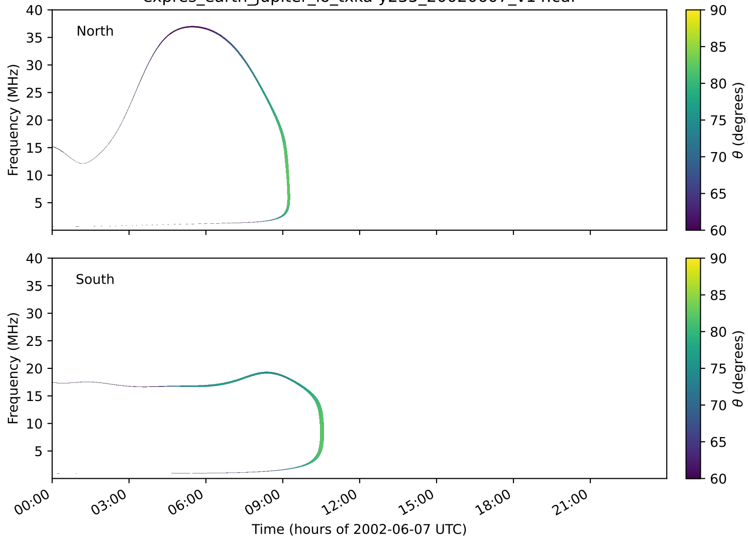
expres_earth_jupiter_io_txka-y235_20020607_v14.cdf
