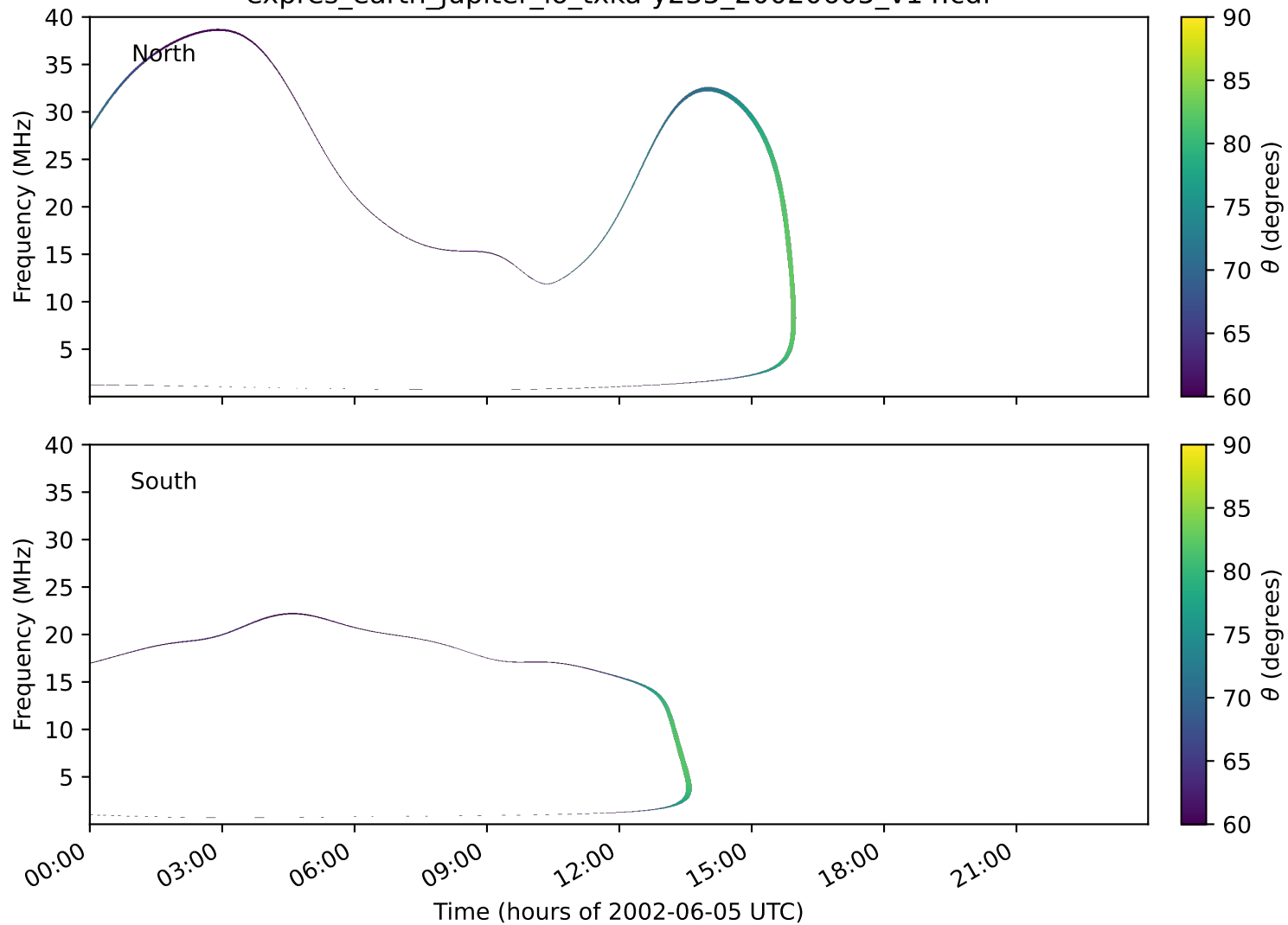
expres_earth_jupiter_io_txka-y235_20020605_v14.cdf
