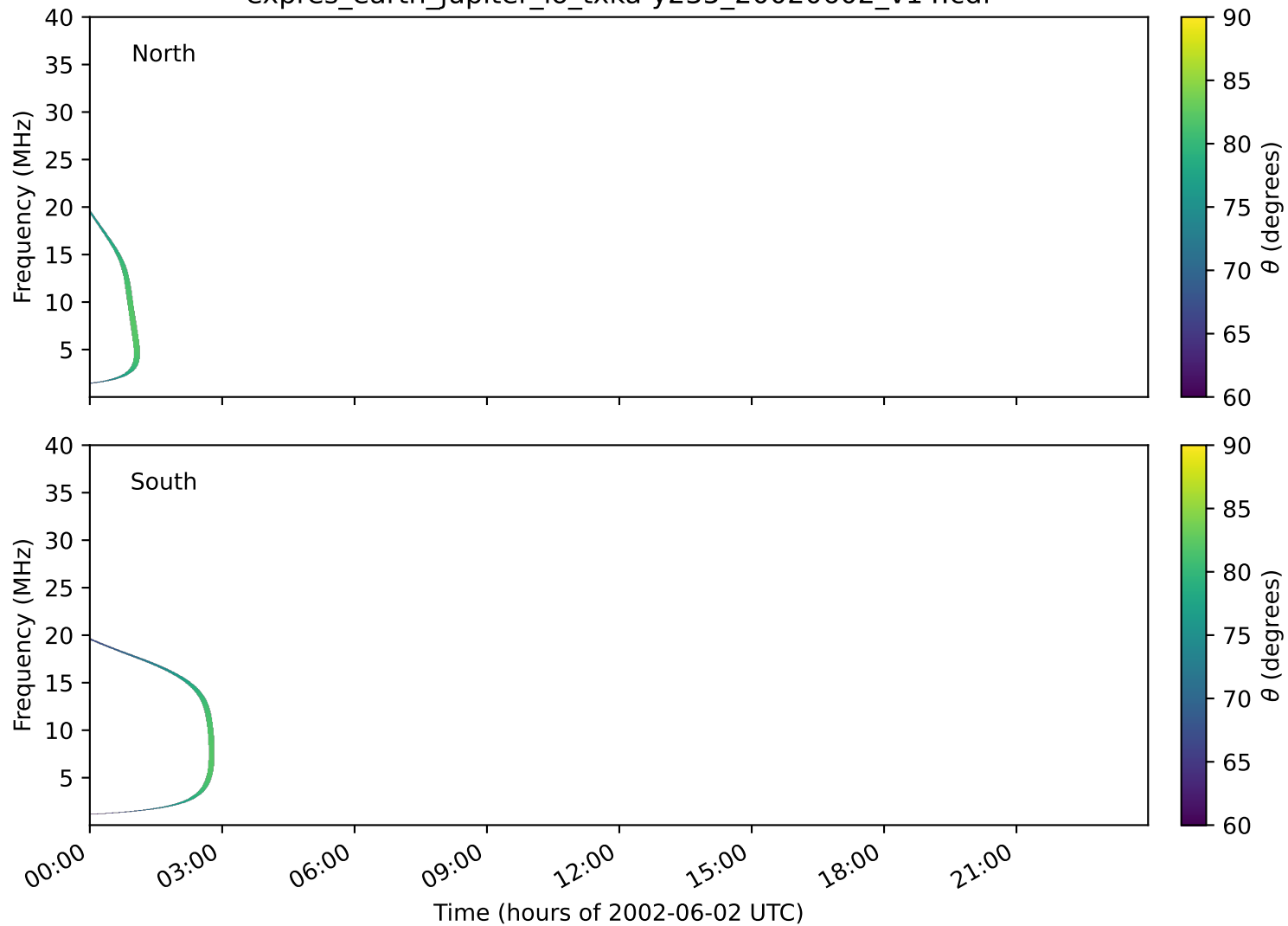
expres_earth_jupiter_io_txka-y235_20020602_v14.cdf
