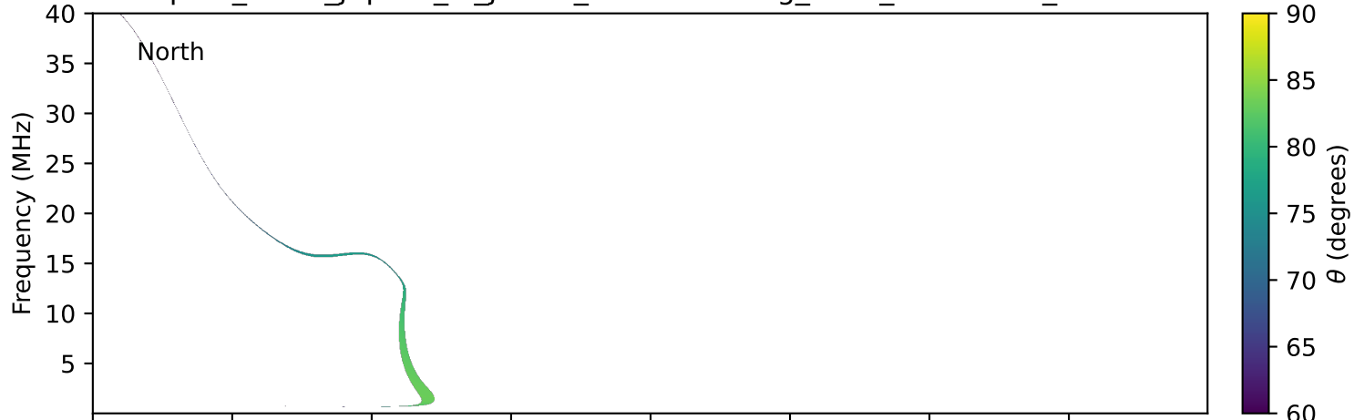
expres_earth_jupiter_io_jrm33_lossc-wid1deg_3kev_20020630_v11.cdf
