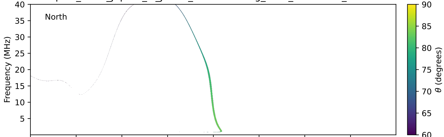
expres_earth_jupiter_io_jrm33_lossc-wid1deg_3kev_20020628_v11.cdf
