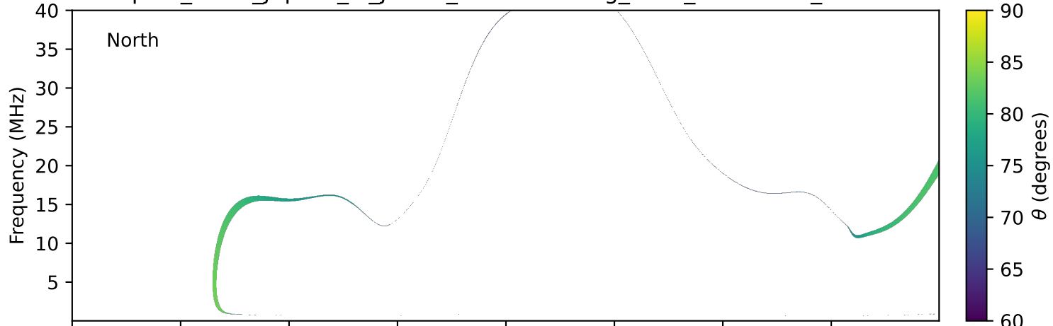
expres_earth_jupiter_io_jrm33_lossc-wid1deg_3kev_20020624_v11.cdf
