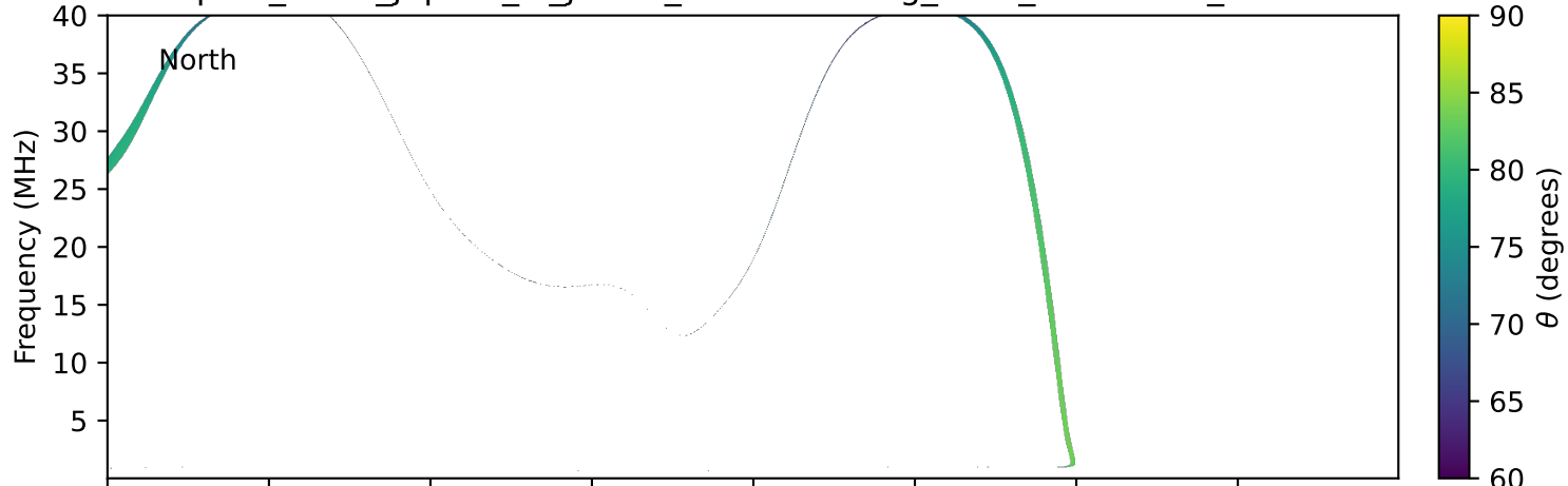
expres_earth_jupiter_io_jrm33_lossc-wid1deg_3kev_20020612_v11.cdf
