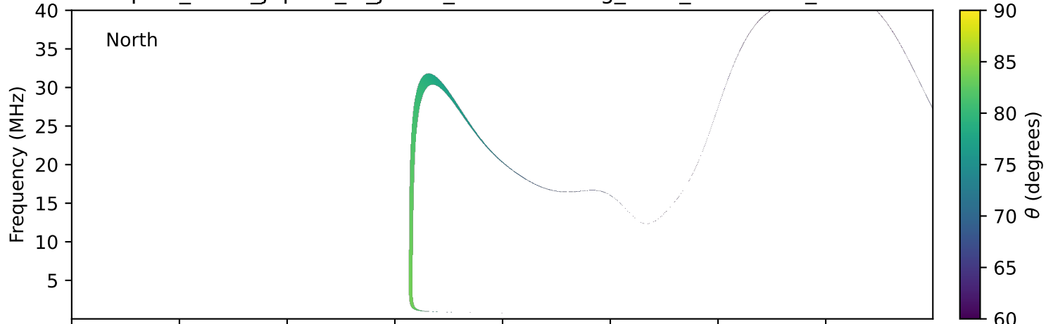
expres_earth_jupiter_io_jrm33_lossc-wid1deg_3kev_20020608_v11.cdf
