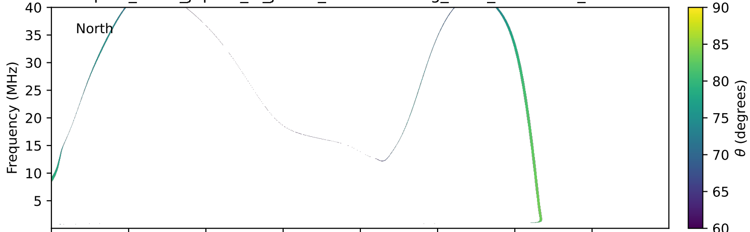
expres_earth_jupiter_io_jrm09_lossc-wid1deg_3kev_20020626_v11.cdf
