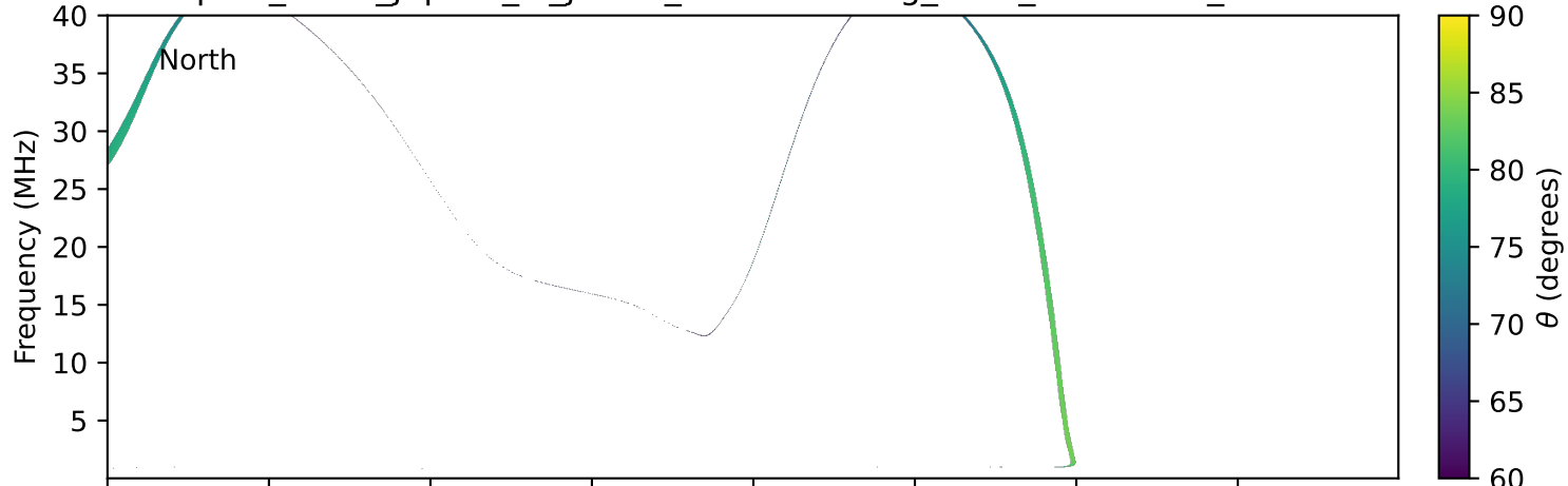
expres_earth_jupiter_io_jrm09_lossc-wid1deg_3kev_20020612_v11.cdf
