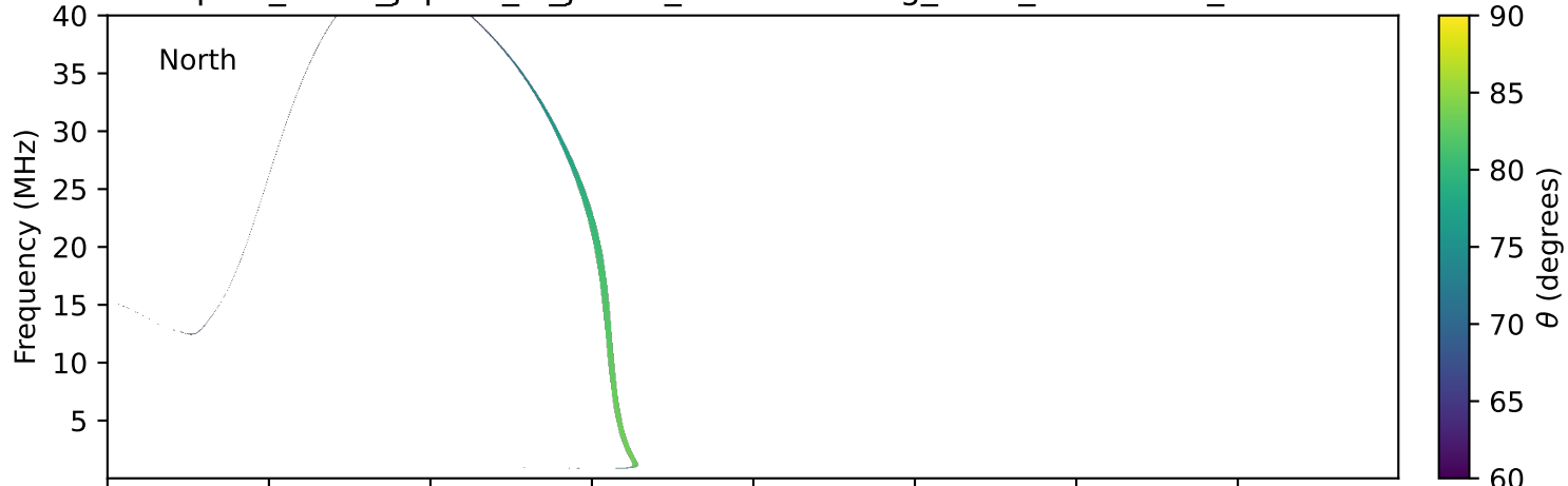
expres_earth_jupiter_io_jrm09_lossc-wid1deg_3kev_20020607_v11.cdf
