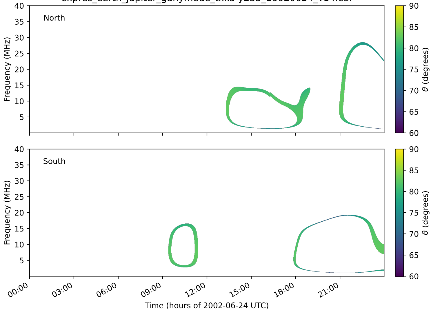
expres_earth_jupiter_ganymede_txka-y235_20020624_v14.cdf
