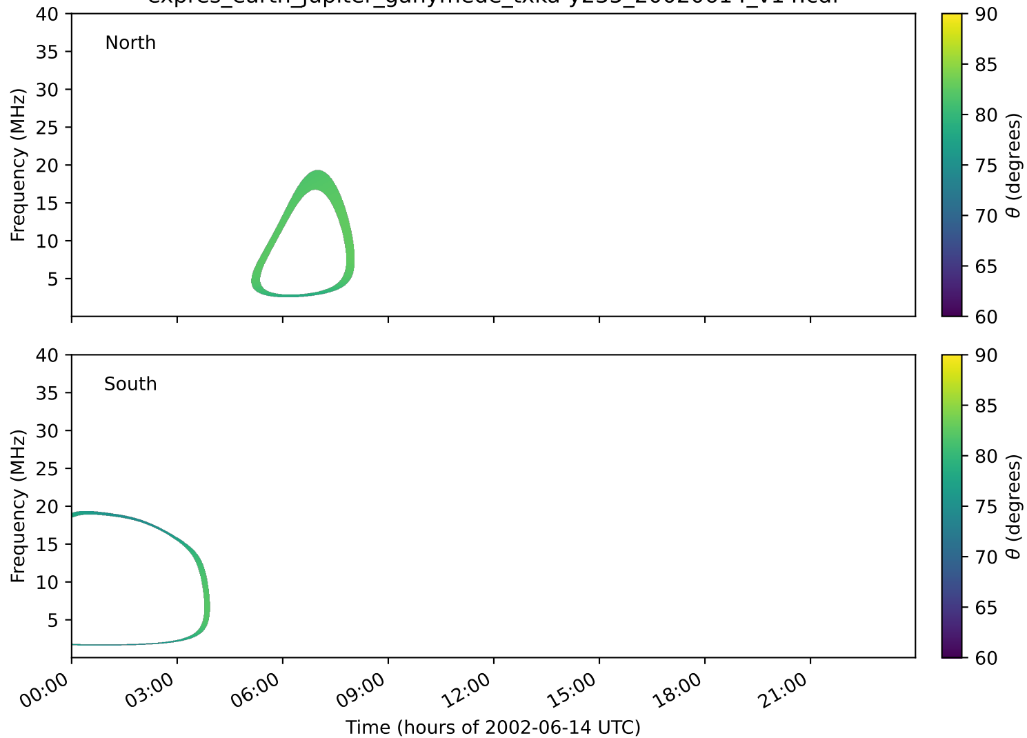
expres_earth_jupiter_ganymede_txka-y235_20020614_v14.cdf
