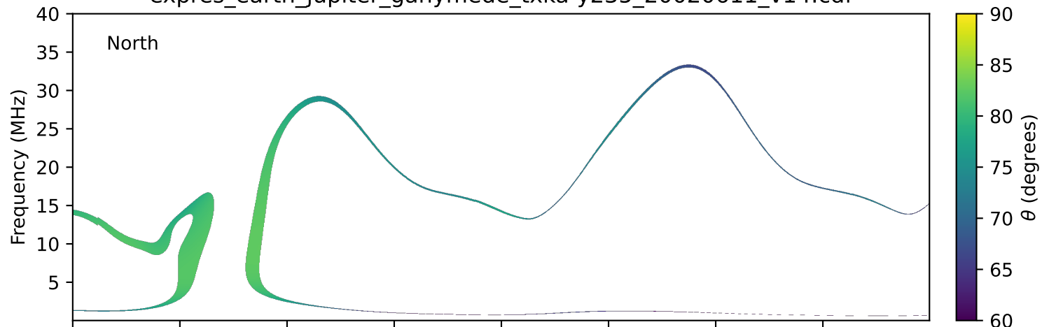
expres_earth_jupiter_ganymede_txka-y235_20020611_v14.cdf
