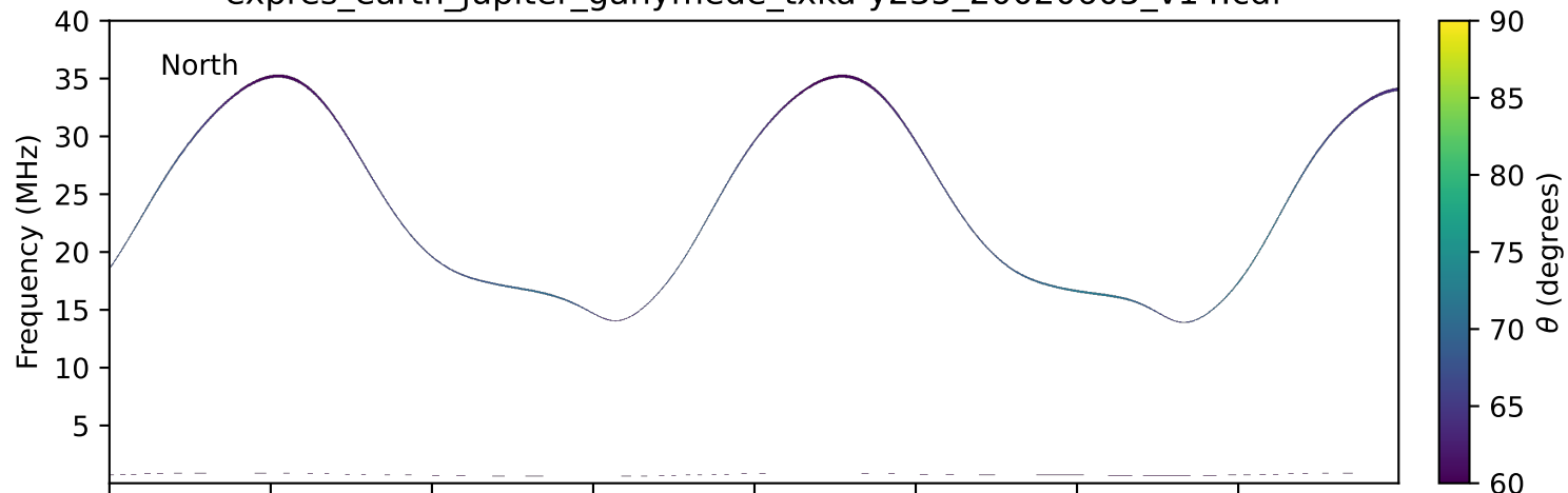
expres_earth_jupiter_ganymede_txka-y235_20020605_v14.cdf
