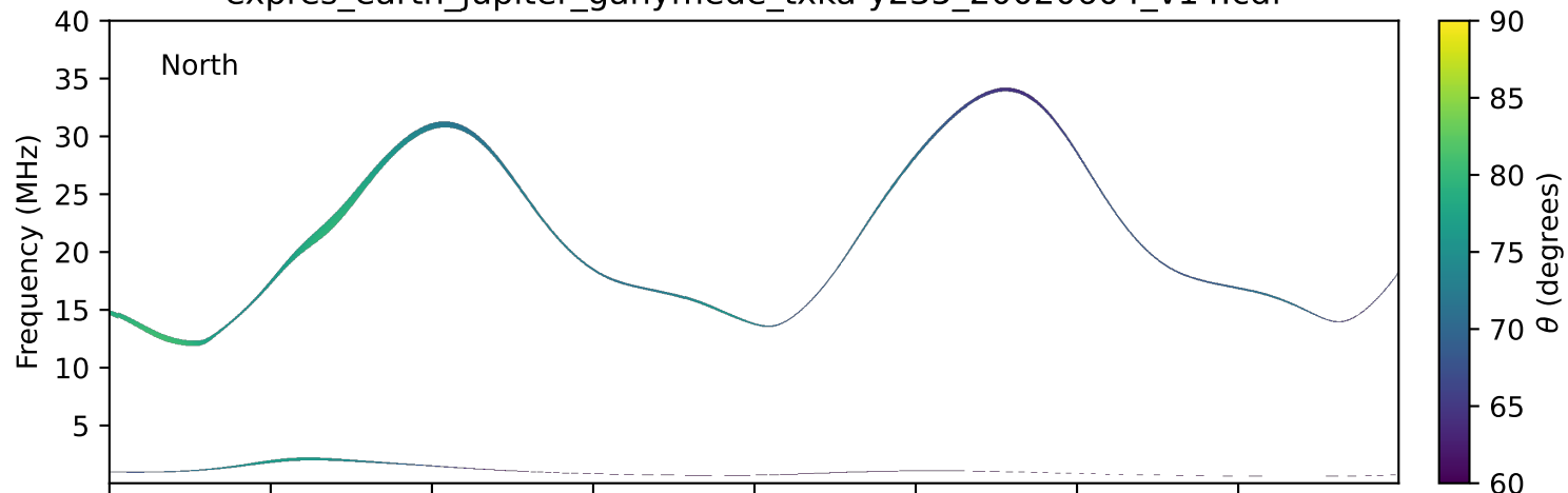
expres_earth_jupiter_ganymede_txka-y235_20020604_v14.cdf
