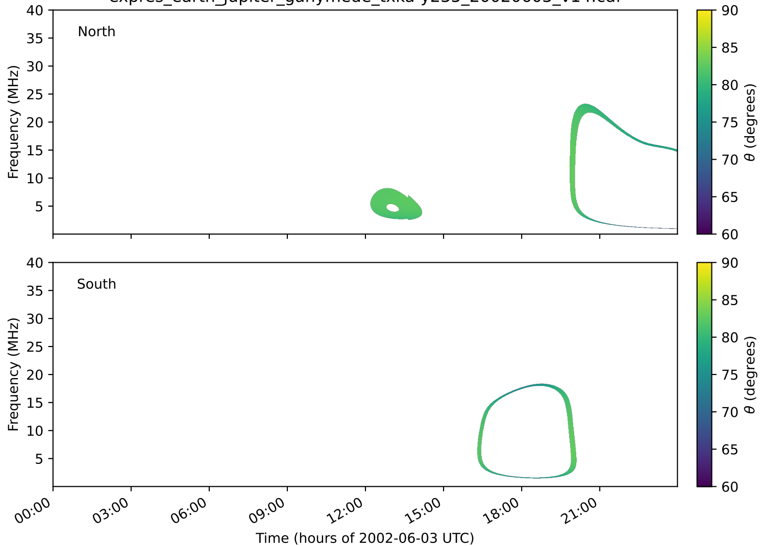
expres_earth_jupiter_ganymede_txka-y235_20020603_v14.cdf
